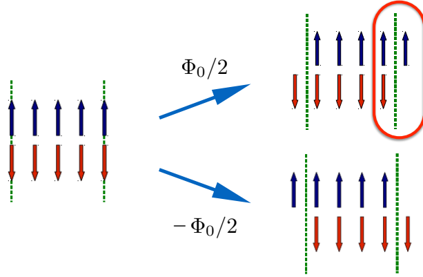
Figure 2.2: Flux insertion in the QSHE: up and down spins are displaced w.r.t. the Fermi surfaces at L and R edges of the annulus (dashed-dotted lines).
