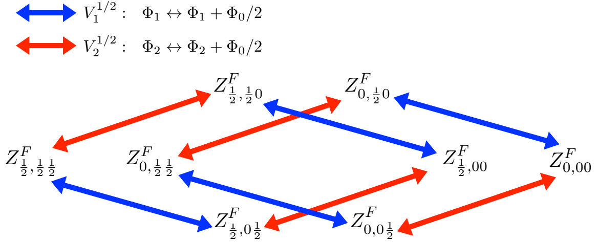
Figure 4.8: Action of V_1^{1/2} and V_2^{1/2} on the eight partition functions Z_{\alpha_0, \alpha_1 \alpha_2}^F , where \alpha_\mu = 0 (1/2) corresponds to periodic (antiperiodic) boundary conditions.
