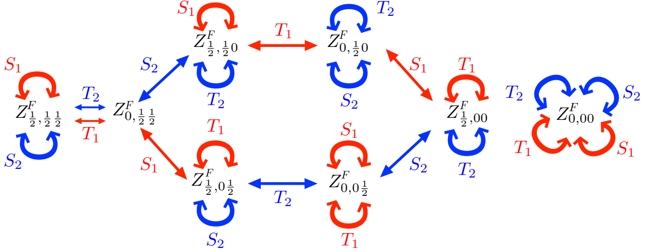
Figure 4.12: Action of the modular transformations T_1 , T_2 , S_1 and S_2 on the eight partition functions Z_{\alpha_0, \alpha_1, \alpha_2}^F . Recall that \alpha_\mu = 0(1/2) for periodic (antiperiodic) boundary conditions.
