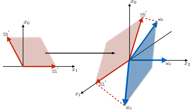
Figure 4.11: Projection of the parallelogram between \omega_0 and \omega_1 on the plane (x_0, x_1) .
