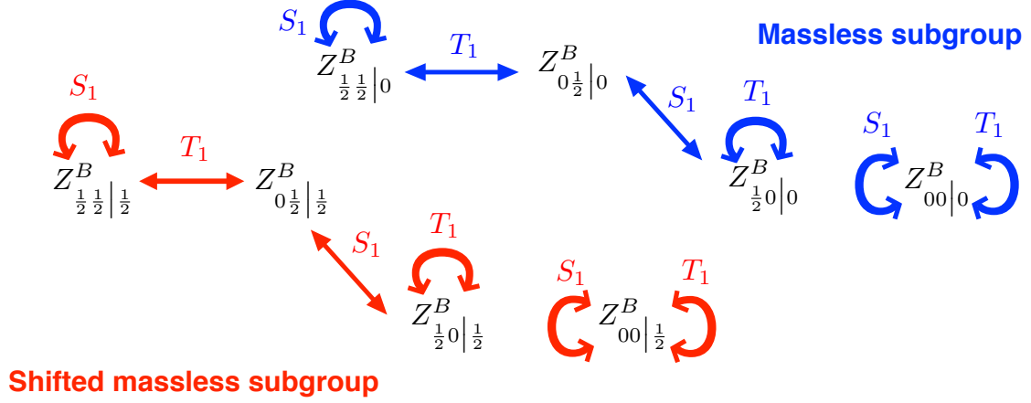
Figure 5.4: Action of the two-dimensional modular group SL(2, \mathbb{Z}) over of the eight bosonic partition functions Z^B_{\alpha_0 \alpha_1 | \alpha_2} reduced on the (x^0, x^1) plane.
