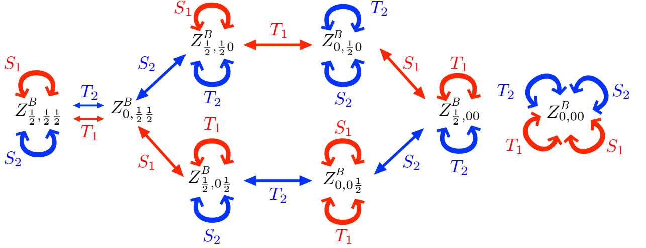
Figure 5.3: Action of SL(3, \mathbb{Z}) over the bosonic partition functions Z_{\alpha_0, \alpha_1 \alpha_2}^B .
