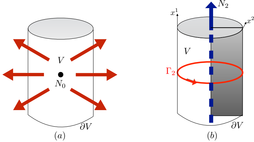
Figure 5.1: The thick two-torus V = D^2 \times S^1 is represented as a filled cylinder with identified faces. (a): The bulk quasiparticle with charge N_0 creates a flux of the b field across the boundary surface \partial V . (b): In blue the bulk vortex of charge N_2 along the non-trivial cycle x^1 , in red the closed line \Gamma_2 encircling on the surface the vortex excitation, in grey the branch cut surface from the vortex excitation to the boundary surface \partial V .
